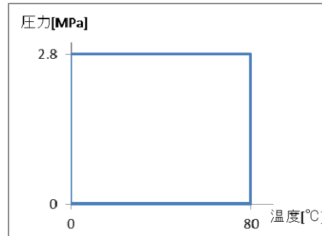
20SWZ, 20SWZU
