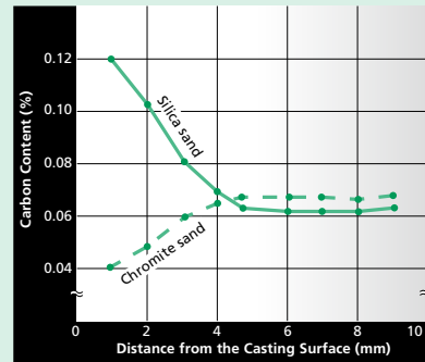
Mold Sands: Decarbonization
