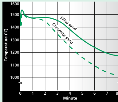
Mold Sands: Cooling Effect
