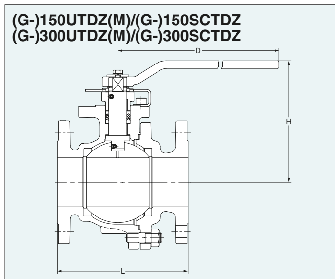
Dimensions of 150UTDZ(M), 150SCTDZ
