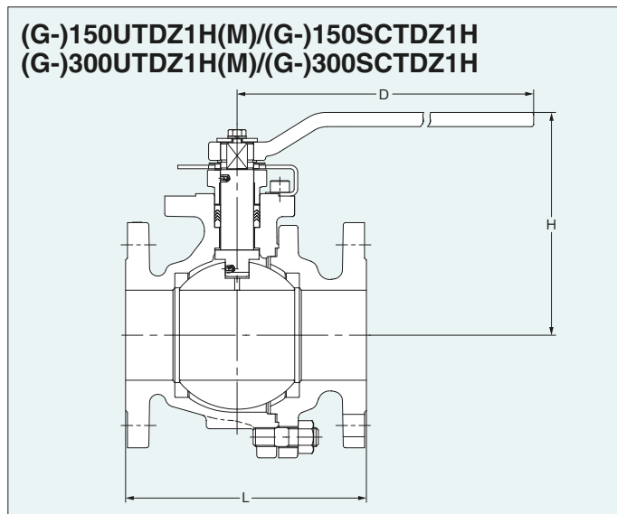
Dimensions of 150UTDZ1H(M), 150SCTDZ1H
