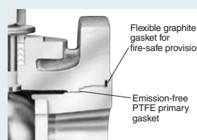
Fig. 9 (Uni-body insert)
