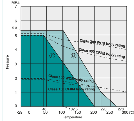
150/300UTAZ(M)/SCTAZM : NPS 1 1/2 to 3
