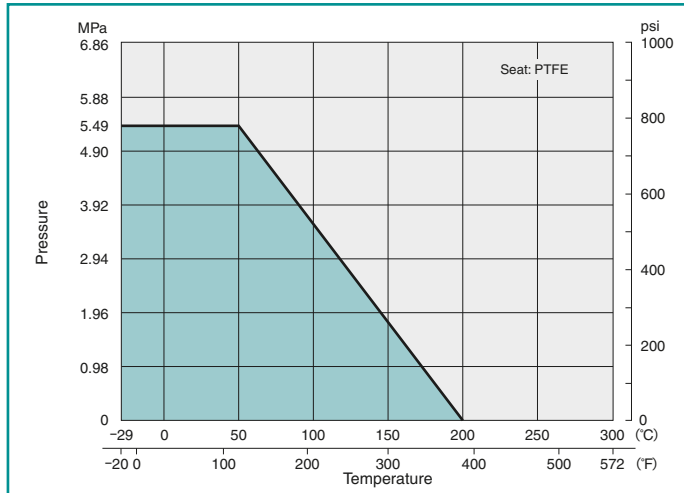
Type 800: UTH(M)
