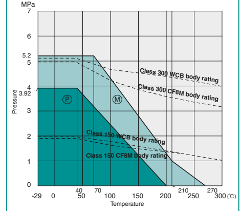
150/300UTAZ(M)/SCTAZM : NPS 4, 6
